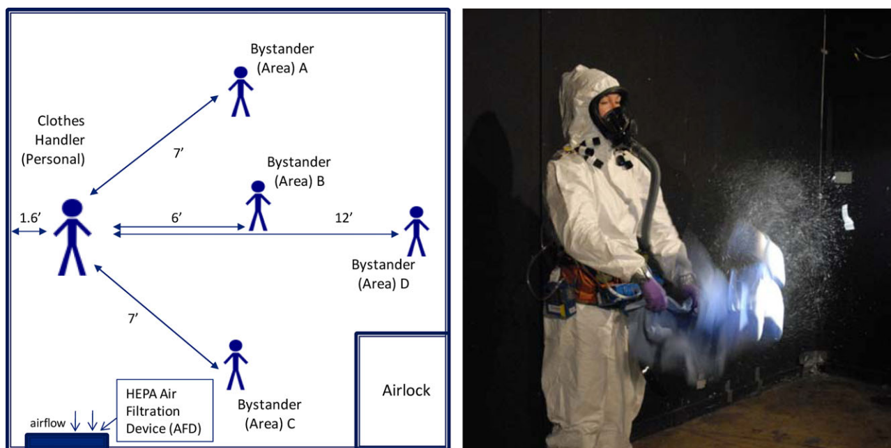
Fig. 1. Depiction of chamber and testing arrangement. Photo depicts person shaking asbestos-contaminated clothing.
